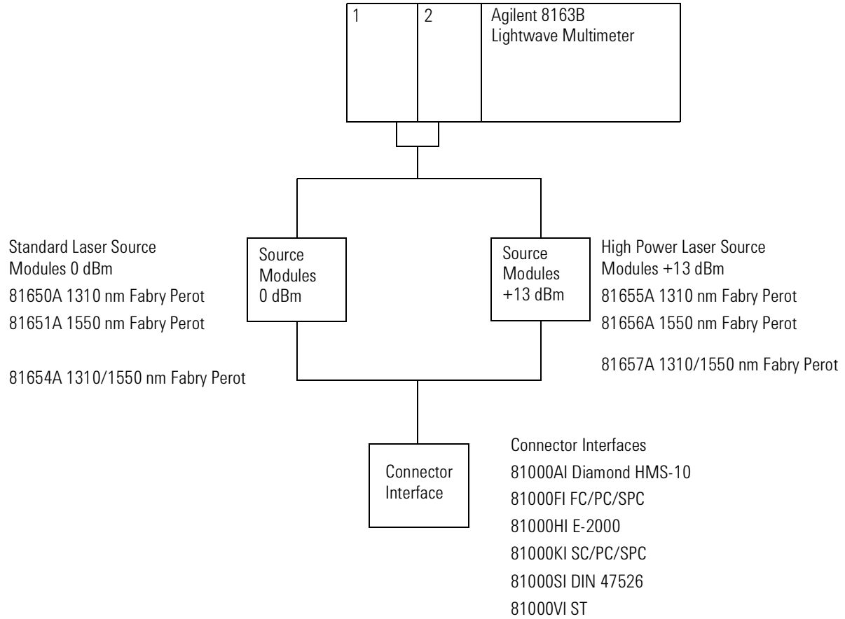
Figure 4 Recommended Connector Interfaces
