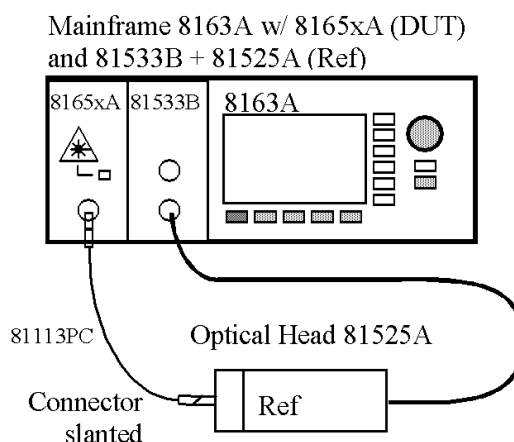
Figure 6 Measurement Setup for Output Power and Stability Test
