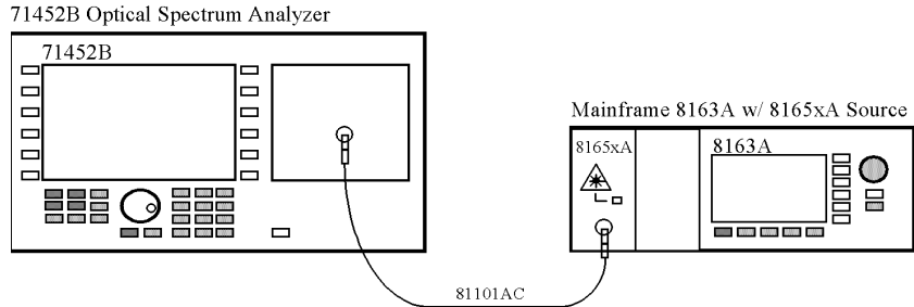
Figure 5 Measurement Setup for Center Wavelength and Spectral Bandwidth
